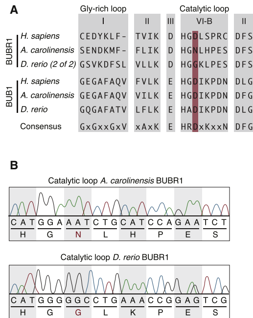
Figure 4. The BUBR1 Orthologs of the Vertebrates A. carolinensis and D. rerio Are Bona Fide Pseudokinases
