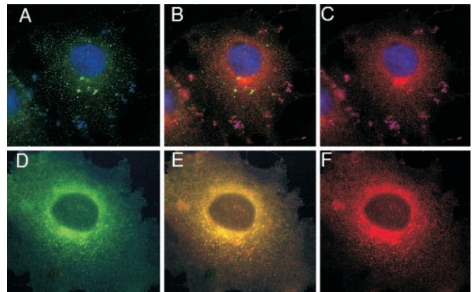
FIG. 4. Localization of tuberin, hamartin, and rabaptin in COS cells. Double label immunofluorescence microscopy was performed on co-transfected COS cells overexpressing hamartin and Xpress-tagged rabaptin (A–C) and tuberin and Xpress-tagged rabaptin (D–F). A, hamartin expression, showing the characteristic punctate labeling pattern in the cytoplasm (green fluorescence). B, combined double label image showing hamartin, as in A (green fluorescence) and rabaptin (red fluorescence). Rabaptin shows the expected diffuse, cytoplasmic labeling pattern, and there is minimal overlap of the hamartin and rabaptin signals. C, rabaptin expression (red fluorescence). D, tuberin expression, showing typical diffuse cytoplasmic staining (green fluorescence). E, combined double label image showing tuberin, as in D (green fluorescence), and rabaptin (red fluorescence). Yellow indicates significant overlap of the tuberin and rabaptin signals. F, rabaptin expression (red fluorescence).
