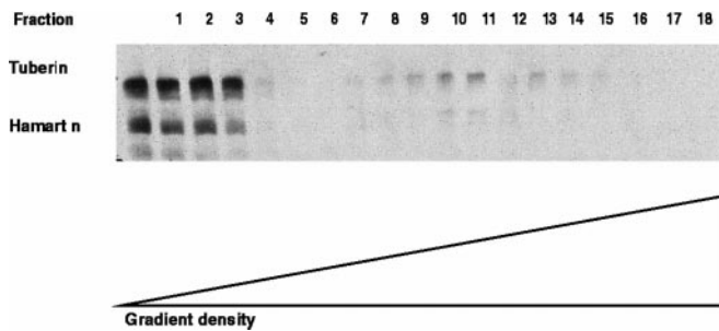
FIG. 2. Flotation gradient centrifugation of tuberin and hamartin. A HeLa cell homogenate was brought to 50% (w/w) sucrose and overlaid with a 15–40% (w/w) sucrose gradient. After centrifugation at 42,000 rpm for 14 h at 4 °C in a Beckman SW50.1 rotor, 0.2-ml fractions were analyzed by immunoblotting. Tuberin and hamartin are indicated. The bar indicates increasing sucrose density.
