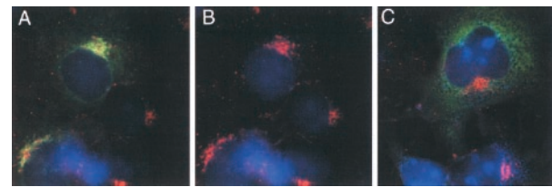
FIG. 3. Localization of tuberin and wheat germ agglutinin in COS cells. A, COS cells transfected with an \alpha -glucosidase expression construct, showing clear overlap between the expression of acid \alpha -glucosidase (green fluorescence) and the distribution of the Golgi complex, as revealed by a wheat germ agglutinin-rhodamine conjugate (red fluorescence). Acid \alpha -glucosidase is transported through the Golgi complex en route to the lysosome. B, same image as in A, without the \alpha -glucosidase signal to indicate the Golgi-specific wheat germ agglutinin signal (red fluorescence). C, COS cells transfected with TSC2. The distribution of tuberin (green fluorescence) is clearly distinct from that of the Golgi marker wheat-germ agglutinin (red fluorescence).
