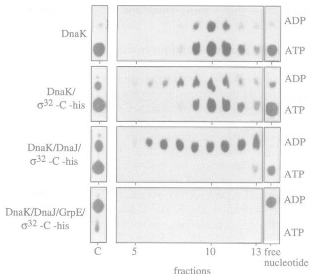
Fig. 7. Identification of nucleotide associated with chaperone- \sigma^{32} -C-his complexes. DnaK (2 \mu M), DnaJ (4 \mu M), GrpE (4 \mu M) and \sigma^{32} -C-his (1 \mu M) as indicated were incubated with [ \alpha - ^{32} P]ATP for 7 min at 30°C and subjected to Superdex 200 gel filtration. Aliquots of the incubation mixture before injection (C) and the eluted fractions including free nucleotide (eluting in peak fraction 25) were analysed by TLC.
