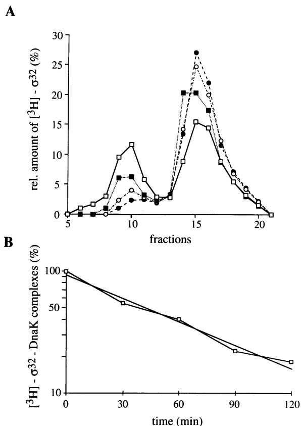
Fig. 1. Stability of DnaK- \sigma^{32} complexes in the absence of ATP. DnaK (4 \mu\text{M} ) and [^3\text{H}]\sigma^{32} (5 \mu\text{M} ) were incubated in 20 \mu\text{l} buffer T for 30 min at 30°C, followed by addition of 180 \mu\text{l} unlabeled \sigma^{32} -C-his (20 \mu\text{M} final concentration in a 200 \mu\text{l} volume). At 1, 30, 60, 90 and 120 min after addition of \sigma^{32} -C-his (chase), samples were immediately subjected to Superdex 200 gel filtration followed by scintillation counting of the eluted fractions. (A) Elution profiles of [^3\text{H}]\sigma^{32} at 1 (□), 30 (■), 60 (○) and 120 (●) min after \sigma^{32} -C-his addition (90 min value not shown). The amount of [^3\text{H}]\sigma^{32} in each fraction is represented as a percentage of the total [^3\text{H}]\sigma^{32} of each run. (B) Chase time-dependent decrease in the amount of [^3\text{H}]\sigma^{32} -DnaK complex. The amount of complex (fractions 8–11) found after 1 min of \sigma^{32} -C-his addition was set as 100%.
