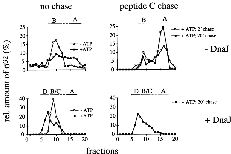
Fig. 2. Stability of chaperone- \sigma^{32} -C-his complexes in the presence of ATP and peptide C competitor. In experiments without DnaJ (upper panel), DnaK (9 \mu M) and \sigma^{32} -C-his (3 \mu M) were incubated for 20 min at 30°C in buffer T without or with ATP (1 mM) and peptide C (30 \mu M), followed by Superdex 200 gel filtration chromatography at 4°C. Peptide C was either added 2 min before injection (2 min chase) or added simultaneously with DnaK to \sigma^{32} -C-his (20 min chase). For samples with ATP the column was pre-equilibrated with buffer T containing 200 \mu M ATP. In experiments with DnaJ (lower panel), DnaK (4 \mu M), DnaJ (4 \mu M) and \sigma^{32} -C-his (1 \mu M) were incubated for 20 min at 30°C in buffer T without or with ATP (1 mM) and peptide C (10 \mu M, 20 min chase) followed by gel filtration. \sigma^{32} -C-his was visualized by immunoblotting with \sigma^{32} -specific antiserum after SDS-PAGE and quantified by densitometric scanning. A, B, C and D indicate the peak fractions of free \sigma^{32} -C-his, DnaK- \sigma^{32} -C-his, DnaJ- \sigma^{32} -C-his and DnaK-DnaJ- \sigma^{32} -C-his complexes respectively.
