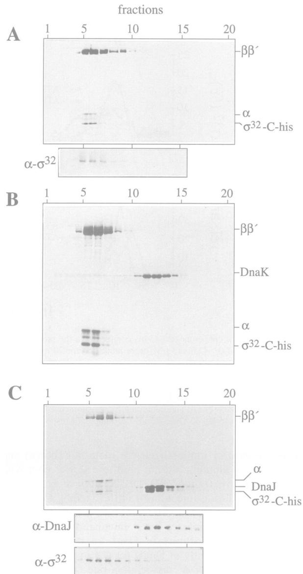
Fig. 4. DnaK and DnaJ do not associate with \sigma^{32} -C-his bound to RNA polymerase. Equimolar concentrations ( 1.5 \mu\text{M} final concentration) of RNAP core and \sigma^{32} -C-his were incubated in buffer T at 30^\circ\text{C} for 10 min. The reactions were further incubated for 20 min at 30^\circ\text{C} with no addition (A) or DnaK (6 \mu\text{M} ) (B) or DnaJ (6 \mu\text{M} ) (C), followed by Superdex 200 gel filtration. Silver stained SDS-PAGE gels with the indicated positions of the \alpha , \beta and \beta' subunits of RNA polymerase are shown. In addition, \sigma^{32} -C-his (A and C) and DnaJ (C) were identified by immunoblot analysis of eluted fractions using \sigma^{32} - or DnaJ-specific antisera.
