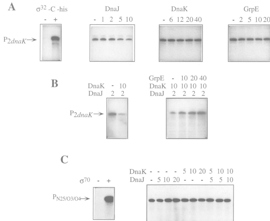
Fig. 8. Control of \sigma^{32} -C-his activity by DnaK, DnaJ and GrpE. In vitro run-off transcriptions are shown from linear DNA templates containing the \sigma^{32} -dependent P_{2dnaK} promoter of the dnaK gene (A and B) and the \sigma^{70} -dependent P_{N25/O3/O4} promoter (C). To transcription assay mixtures containing RNAP core and \sigma^{32} -C-his (A and B) or \sigma^{70} (C) were added DnaK, DnaJ and GrpE at the indicated molar excesses with respect to \sigma^{32} -C-his or \sigma^{70} . Transcripts were analyzed by polyacrylamide-urea gel electrophoresis followed by autoradiography.
