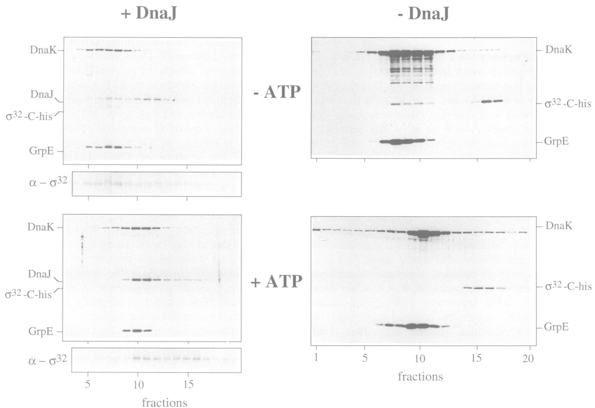
Fig. 6. GrpE allows formation and ATP-mediated dissociation of quaternary GrpE–DnaK–DnaJ– \sigma^{32} -C-his complexes. (Left) DnaK, DnaJ, GrpE and \sigma^{32} -C-his (final concentrations of 2, 4, 4 and 1 \mu M respectively) were incubated for 20 min at 30°C in buffer T containing ATP (1 mM), followed by gel filtration using a Superdex 200 column equilibrated in running buffer with or without 200 \mu M ATP. Eluted proteins were separated by SDS-PAGE and visualized either by silver staining or, for \sigma^{32} -C-his, immunoblot analysis with \sigma^{32} -specific antiserum. (Right) DnaK, GrpE and \sigma^{32} -C-his (9, 18 and 3 \mu M final concentrations respectively) were incubated and analyzed as described above. \sigma^{32} -C-his is poorly visualized by silver staining.
