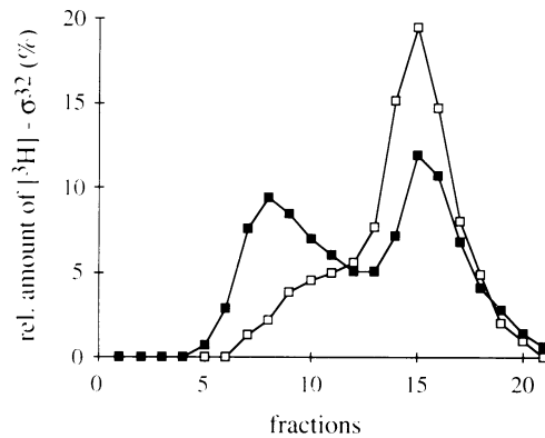
Fig. 5. Stability of DnaK–DnaJ– \sigma^{32} complexes in the presence of ATP. DnaK (8 \mu M), DnaJ (8 \mu M) and [ ^3 H] \sigma^{32} (4 \mu M) were incubated in 20 \mu l buffer T at 30°C. After 30 min 180 \mu l buffer T without (■) or with \sigma^{32} -C-his (□, 20 \mu M final concentration) was added and immediately transferred onto ice and injected into a Superdex 200 gel filtration column. The [ ^3 H] \sigma^{32} in each fraction was determined by scintillation counting and is represented as a percentage of total [ ^3 H] \sigma^{32} of each run.
