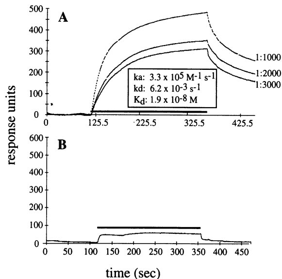
Fig. 3. Surface plasmon resonance analysis of DnaJ association with \sigma^{32} . The resonance signals are plotted as a function of time (s). The amount of protein associating/dissociating from the surface over time was measured in resonance units (RU). The bars in each panel display the time during which the protein was injected. (A) DnaJ in concentrations ranging from 1.1 \times 10^{-7} to 3.7 \times 10^{-8} \text{ M} was injected over immobilized \sigma^{32} . Normalized curves for 1:1000, 1:2000 and 1:3000 dilutions of a 110 \mu\text{M} solution of DnaJ are plotted. (B) Bovine serum albumin was injected over immobilized \sigma^{32} .
