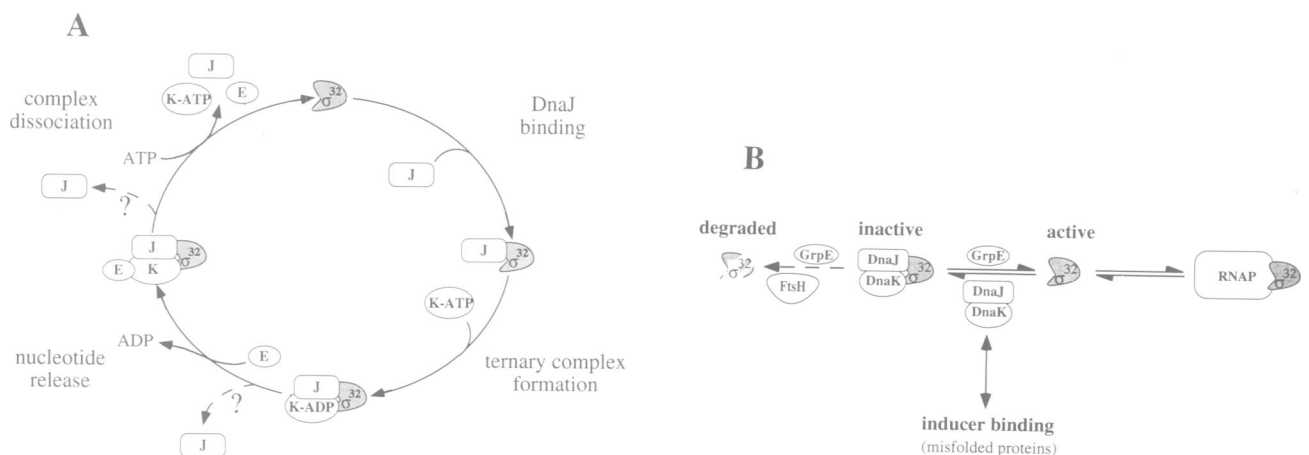
Fig. 9. Homeostatic control of \sigma^{32} activity and stability by a chaperone binding/release cycle. (A) Model of the chaperone binding/release cycle. The cycle starts with rapid association of DnaJ (J) with \sigma^{32} . DnaK (K), in its ATP-bound form, interacts with \sigma^{32} only transiently. DnaJ associated with \sigma^{32} interacts with DnaK-ATP and, through rapid stimulation of ATP hydrolysis by DnaK, targets DnaK to \sigma^{32} , promotes DnaK binding to \sigma^{32} and mediates efficient formation of DnaK-DnaJ- \sigma^{32} complexes containing ADP. GrpE (E) can associate with the DnaK component of this complex, thereby triggering nucleotide release and forming quaternary GrpE-DnaK-DnaJ- \sigma^{32} complexes lacking nucleotide. Spontaneous nucleotide release in the absence of GrpE might also occur, but is considered less important, given that GrpE has an essential role in \sigma^{32} regulation in vivo . Binding of ATP induces complex dissociation. It is possible that DnaJ dissociates from ternary or quaternary complexes independently of DnaK, thereby allowing it in principle to act in this cycle in substoichiometric amounts. (B) Model of chaperone-mediated homeostatic control of \sigma^{32} activity and stability. \sigma^{32} exists either as an active free form that can assemble with RNAP to direct heat shock gene transcription or as an inactive form bound to DnaJ and DnaK. Inactive \sigma^{32} can be activated by chaperone dissociation mediated by GrpE-stimulated nucleotide exchange. \sigma^{32} can be eliminated through DnaK-, DnaJ- and GrpE-dependent degradation by FtsH (Herman et al. , 1995; Tomoyasu et al. , 1995) and perhaps additional proteases. During induction of the heat shock response the equilibrium is shifted towards active \sigma^{32} through sequestering of the DnaK system by binding to misfolded proteins. Upon protein damage repair the DnaK system becomes available and the homeostatic balance is re-established. Elements of this model, in particular the sequestering of chaperones through binding to misfolded proteins, have been described earlier (Craig and Gross, 1991; Bukau, 1993; Yura et al. , 1993).
